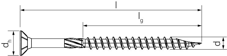
Fig. 1 STR screw (countersunk head)
