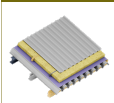
Double-sheet profile roof | see page 64
