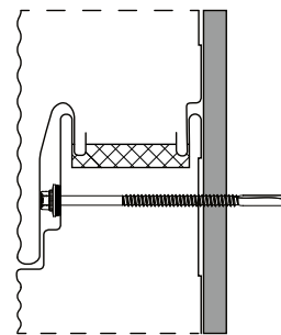
Fig. 1 Not visible sandwich panel installation
