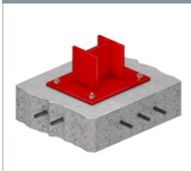
Installation into concrete | see page 314
