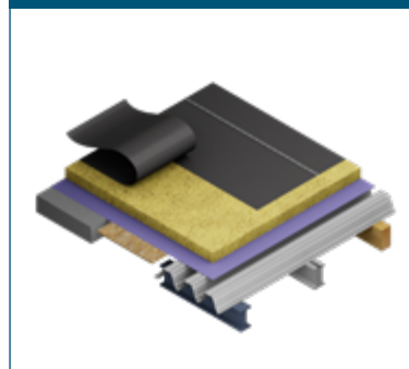
Flat roof with roofing membrane | see page 208
